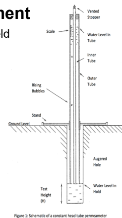
Figure 1: Schematic of a constant head permeameter
