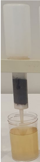
Figure 2. Soil column set-up
