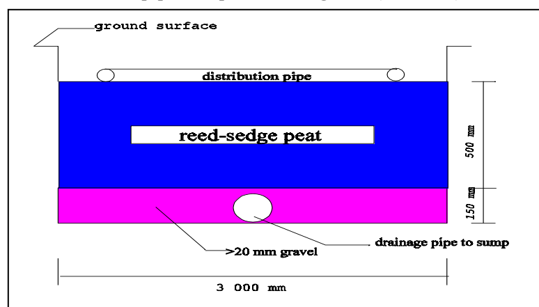
Figure 2 Cross section of peat bed
