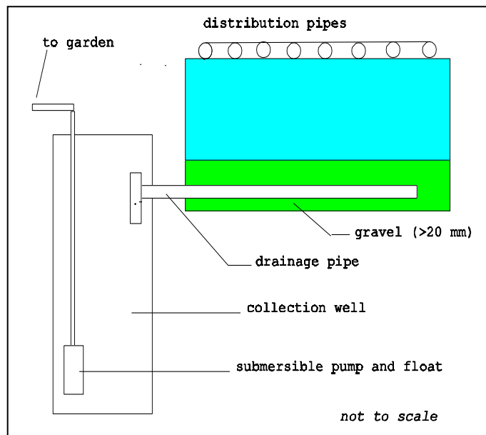
Figure 3 Side elevation of peat bed
