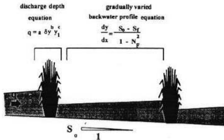
Figure 4: Hydraulic model of flooding through Vetiver hedges
