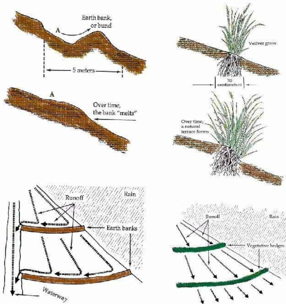
Figure 1: Above left: contour bank; below left: banks divert the water; above right: Vetiver grass create banks or terraces over time; below right: Vetiver hedges slow the runoff to increase infiltration, and the water remains in the field (Greenfield 1989)
